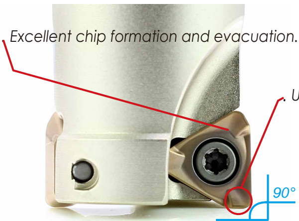
. True 90° square shoulder angle.
